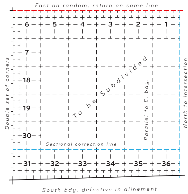
Figure 3-20. Rectification of a south boundary defective in alinement where both the south and west boundaries are fixed in position.
