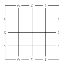
Figure 4-7. Key for marks on special meander corners.
