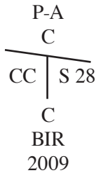
Figure 4-8. Key for marks on closing subdivision-of-section corners.
