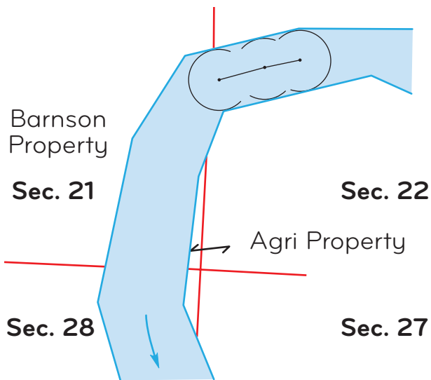
Figure 8-8. The center point of a series of inscribed circles on a straight reach.
